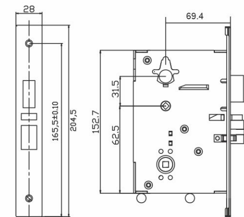
Mortise Body Dimension
