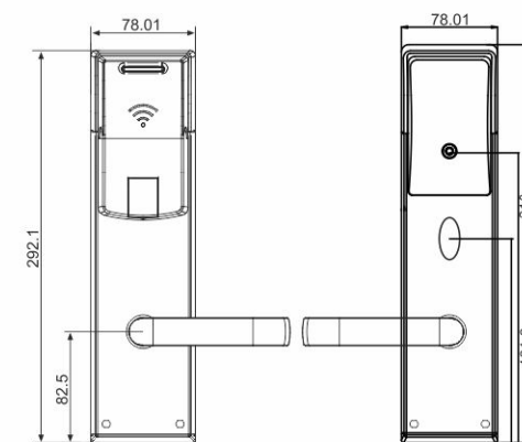
Lock Body Dimension
