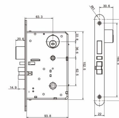
Mortise Body Dimension
