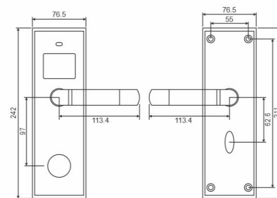
Lock Body Dimension
