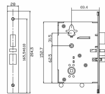
Mortise Body Dimension
