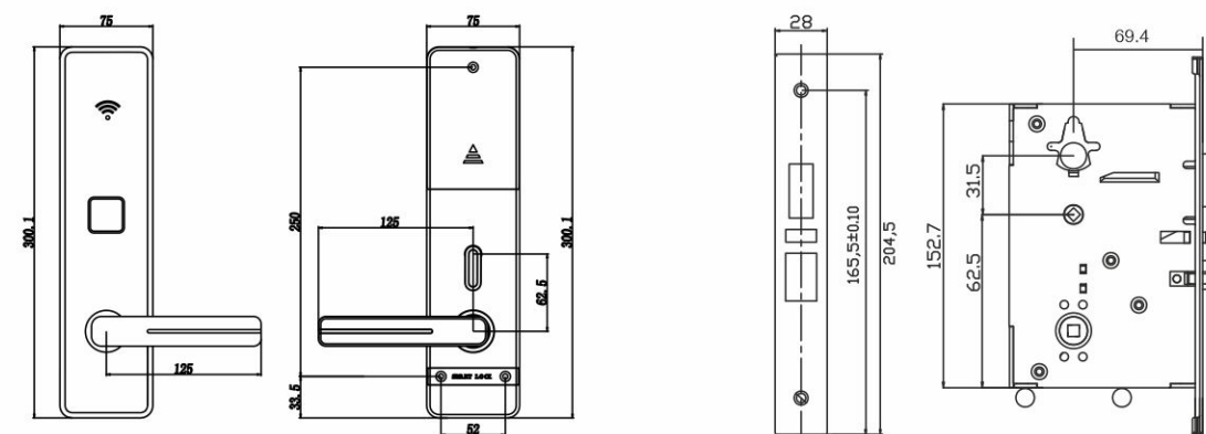
Lock Body Dimension
